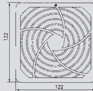
PFG-12 (For UF12A, 12B Series)
