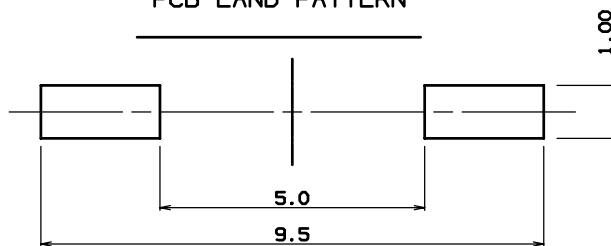
PCB LAND PATTERN
