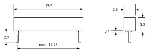
MK with integrated resistor
