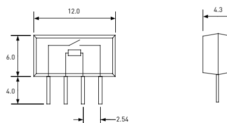
MK with integrated resistor
